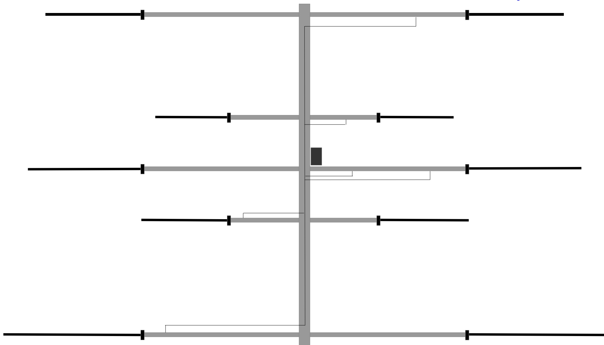
Composition of the 3 elements Duo HB9CV
